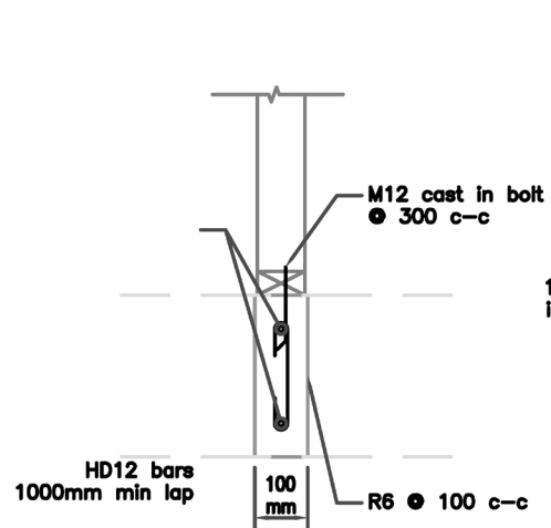
SECTION X-X
